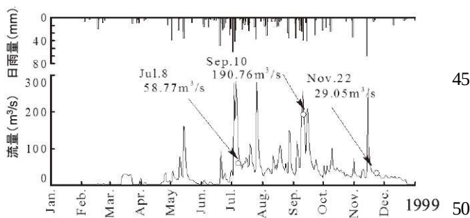
図－1 雨量と流量の関係 1) Fig. 1 Relationship between rainfall and runoff
